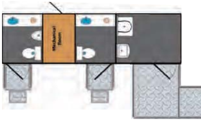
UNIT DIMENSIONS L: 24' W: 14' H: 10'6"
